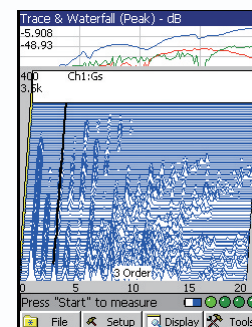
Order tracking: waterfall and trace plot
