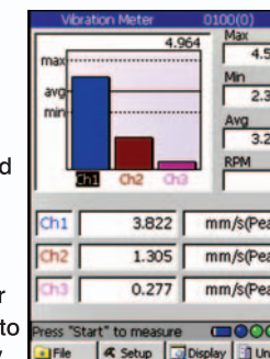
3 channel vibration meter
