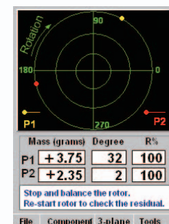
Balancing data and polar plot
