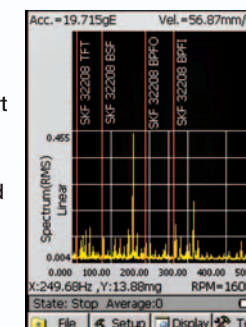
Demodulated spectrum and bearing frequencies
