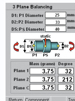
3 plane balancing
