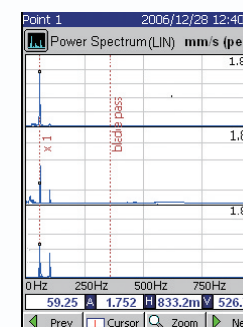
Triaxial spectrum plots
