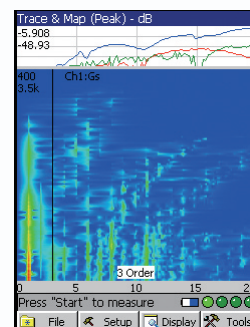
Order tracking: intensity map and traces
